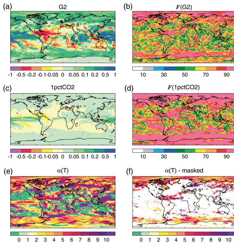
Figure 6. (a)–(d) As in Figure 5 but for the rate of change of annual-mean precipitation rate (mm day -1 per decade). (e) As in Figure 5 but also including negative values which indicate areas where the changes in G2 and 1pctCO2 are of opposite sign. (f) As in Figure 5.
